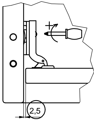
A (1:2)
