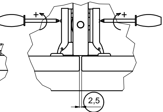
D (1:2)
