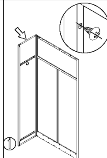
① Connect the left side plate with back plate by self-tapping screws(5x12).
